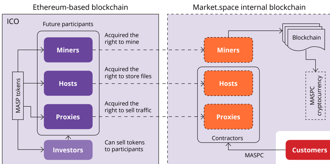
Figure 9. The difference between MASP and MASPC
